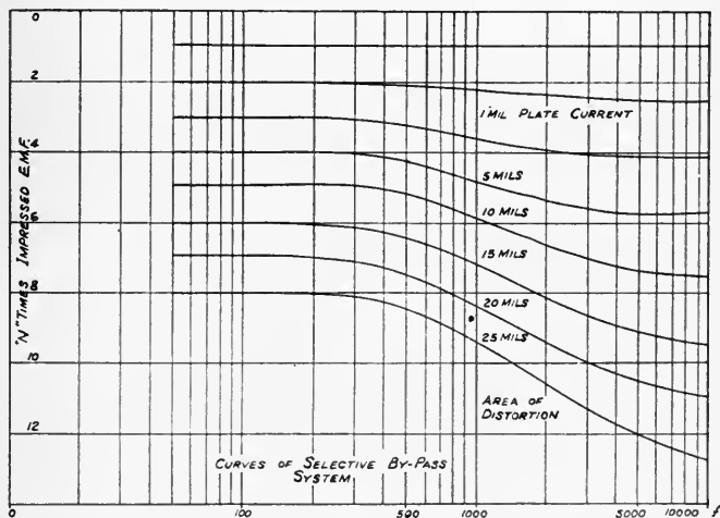
FIG. 7. Curves of selective by-pass system.
